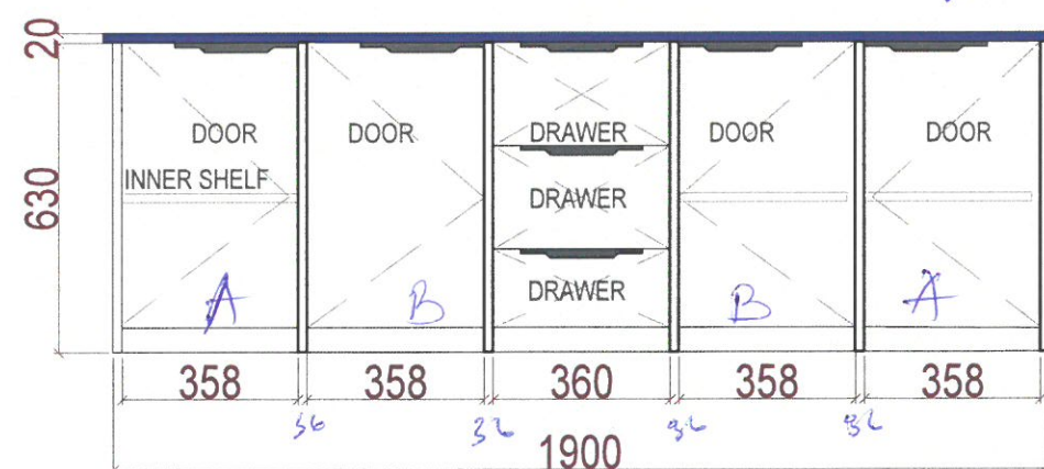
FRONT VIEW CREDENZA- WITH MARBLE STONE TOP MANAGING DIRECTOR'S OFFICE
