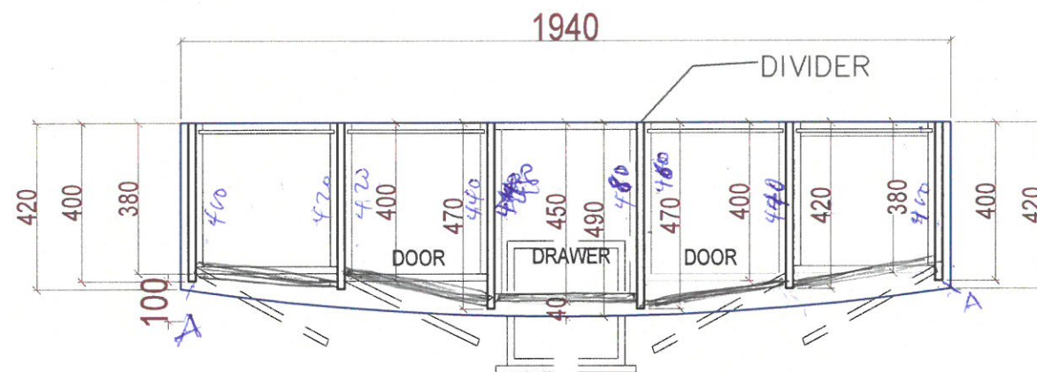
TOP VIEW CREDENZA- WITH MARBLE STONE TOP MANAGING DIRECTOR'S OFFICE
